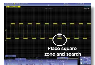
Search for waveforms that pass through/do not pass through a rectangular zone placed on screen.
