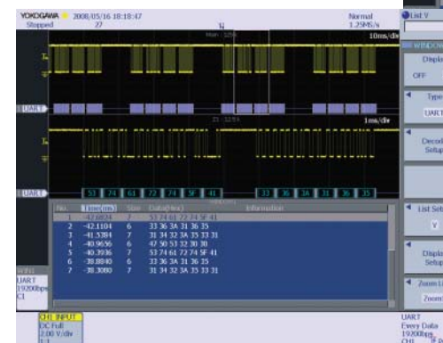
Figure.15 UART trigger setting example
