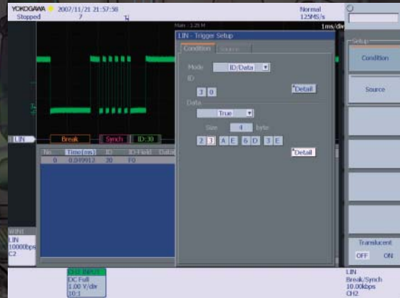
Figure.11 LIN trigger setting example
