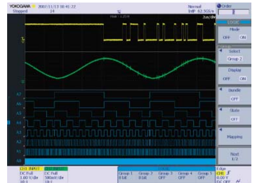
Figure.22 Example of simultaneous observation of analog & logic signals
