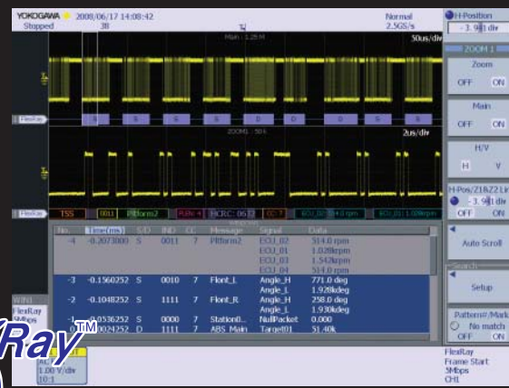
Figure.2 FlexRay FIBEX symbolic decode, analysis list display example
