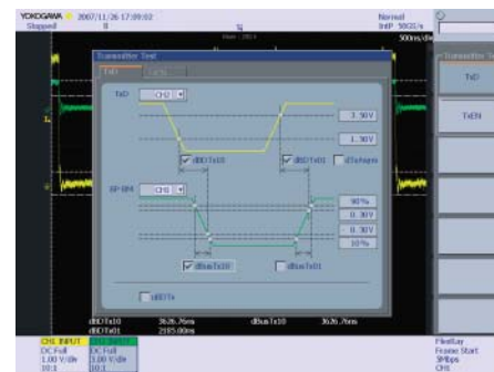
Figure.5 Example of electrical characteristics parameters of the FlexRay bus driver
