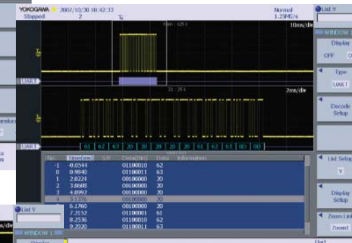
Figure.16 UART waveform, list, decode display example 1
