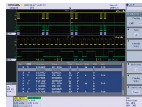
Figure.19 I 2 C waveform, list, decode display example
