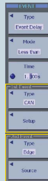
Figure.14 Event Interval Trigger setting example
