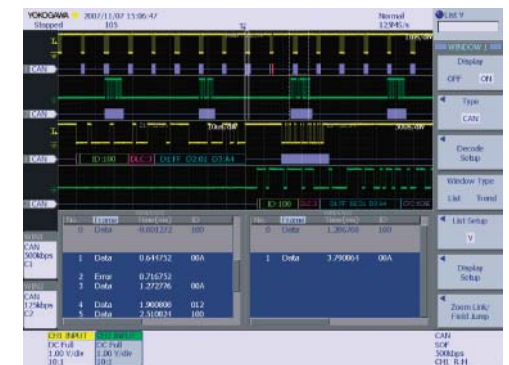
Figure.8 Example of 2-bus simultaneous waveform & decode display
